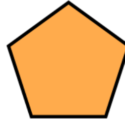
pentagon 5 Sides
