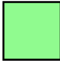
quadrilateral 4 Sides
