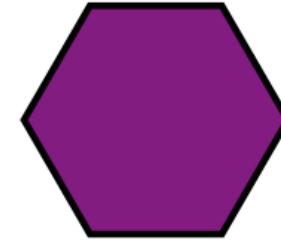
hexagon 6 Sides
