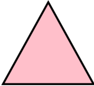
triangle 3 Sides
