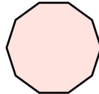
decagon 10 Sides
