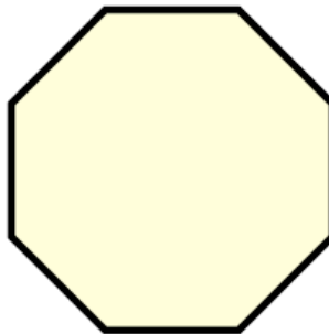
octagon 8 Sides
