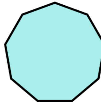
nonagon 9 Sides
