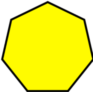
heptagon 7 Sides
